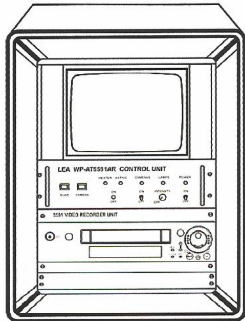
WP-AT5591AR UVIS Rack mounted command center with 14" color monitor and Jog Shuttle VCR
